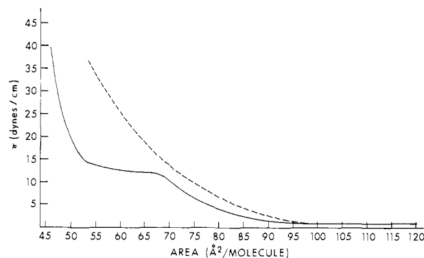
Figure 1. Force-area isotherms for L-DPPC at the air-water (pH 5.5) interface at 25 \pm 0.2 (—) and 44.5 \pm 0.5^\circ (---). The isotherm shown is for a compression rate of 7.2 \text{ \AA}^2/\text{molecule}/\text{min} . Compression rates of 18.0 and 27.7 \text{ \AA}^2/\text{molecule}/\text{min} were also used, giving the same results as shown here.
