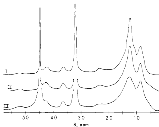
Figure 5. Proton magnetic resonance spectra of D_2O vesicles prepared from L-DPPC alone (I) and combined with epicholesterol (20%, II; 50%, III). Spectra obtained as described in Figure 4.
