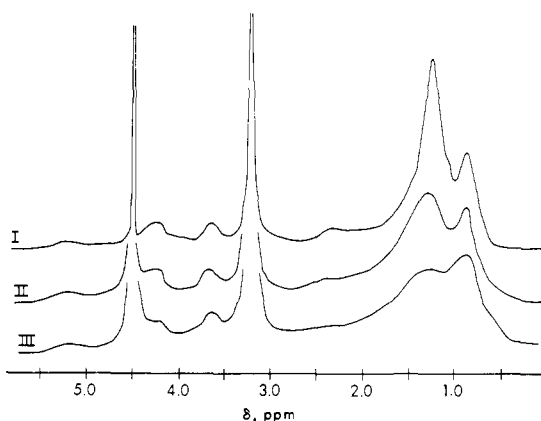
Figure 4. Proton magnetic resonance spectra of D_2O vesicles prepared from L-DPPC alone (I) and combined with cholesterol (20%, II; 50%, III). Spectra were obtained at 52^\circ C on a JEOL-FX90Q spectrometer.
